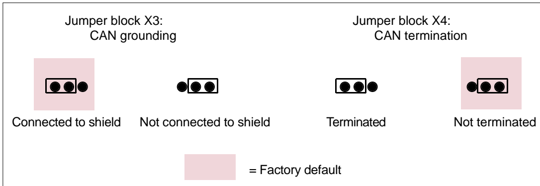
Figure 3-19. Jumper selections for OPT-D6
