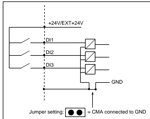
Figure 1-4. If CMA is connected to GND with inboard jumper the internal +24V is used and the CMA terminal ed not be wired
